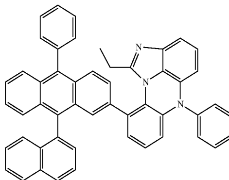
[Chemical Formula 8-22]
