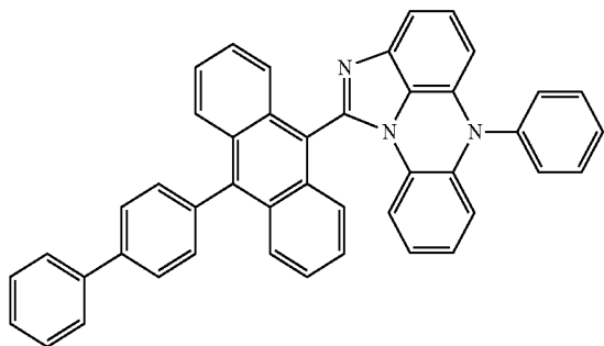
[Chemical Formula 5-4]
