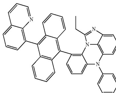
[Chemical Formula 8-11]
