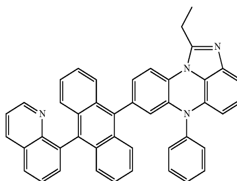
[Chemical Formula 3-11]
