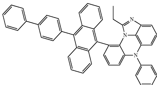
[Chemical Formula 8-4]
