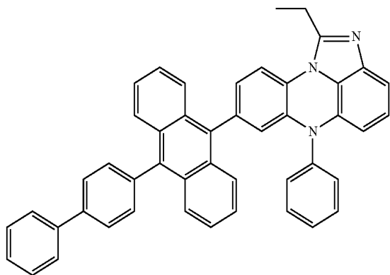
[Chemical Formula 3-5]
