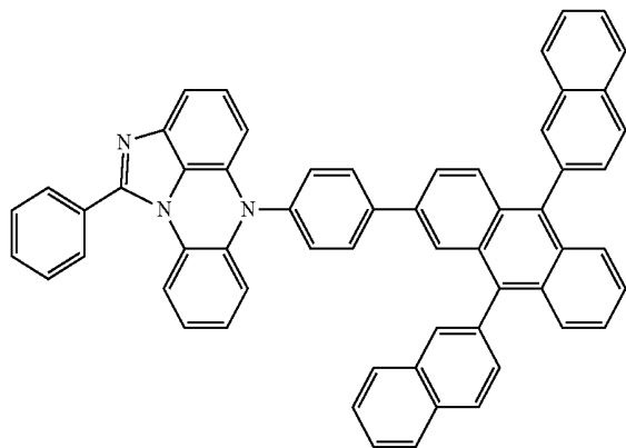
[Chemical Formula 12-25]
