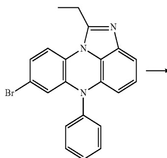
[Compound 2-A]
