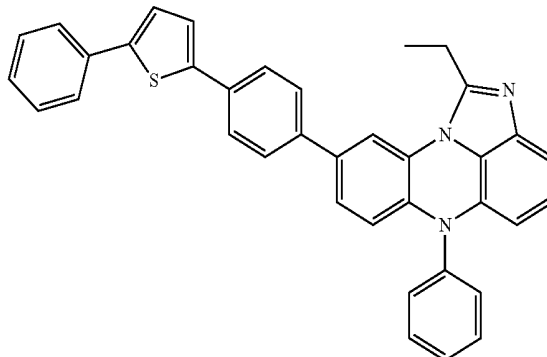
[Chemical Formula 7-39]
