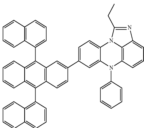
[Chemical Formula 3-21]
