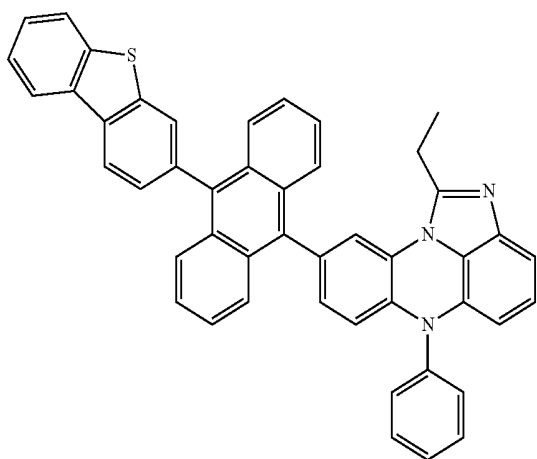
[Chemical Formula 7-14]
