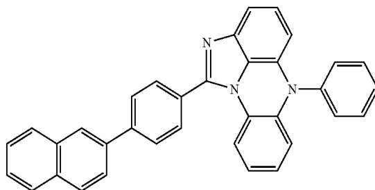
[Chemical Formula 5-27]
