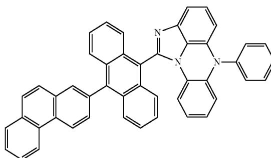
[Chemical Formula 5-9]
