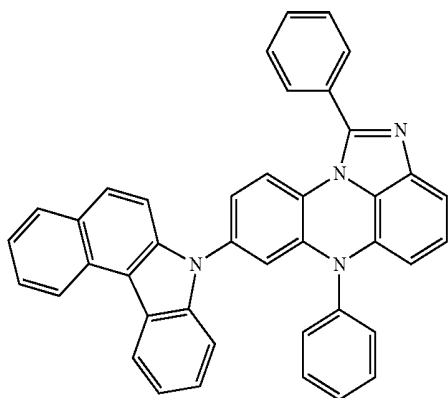
[Chemical Formula 4-51]
