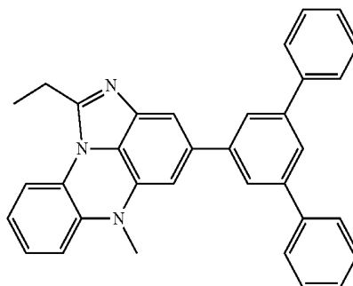
[Chemical Formula 10-5]
