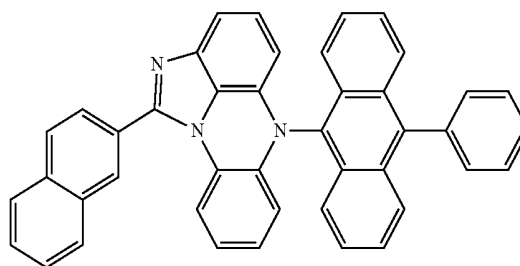
[Chemical Formula 12-1]
