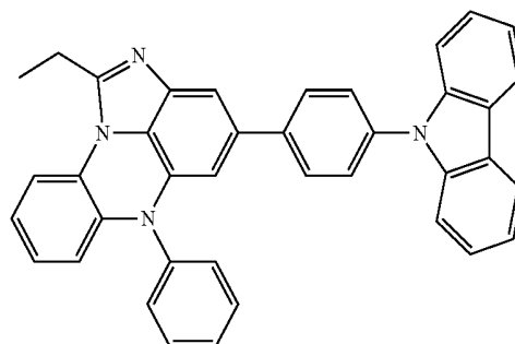
[Chemical Formula 10-6]
