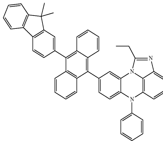
[Chemical Formula 7-5]
