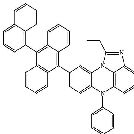
[Chemical Formula 7-3]
