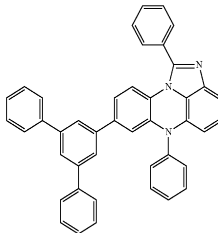
[Chemical Formula 4-40]
