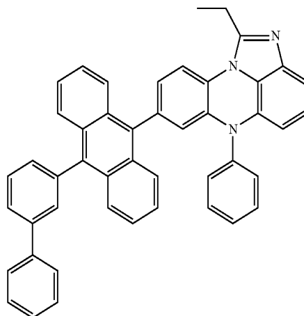
[Chemical Formula 3-6]
