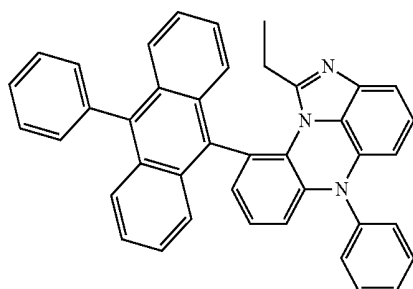
[Chemical Formula 8-1]
