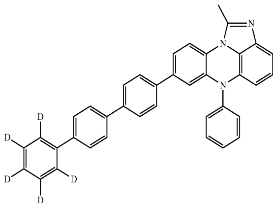
[Chemical Formula 2-52]
