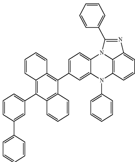
[Chemical Formula 4-6]
