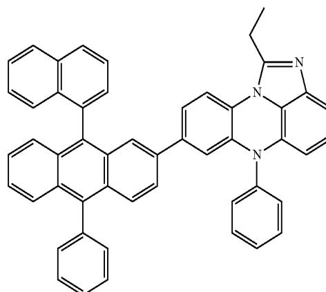
[Chemical Formula 3-22]
