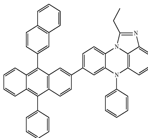
[Chemical Formula 3-23]
