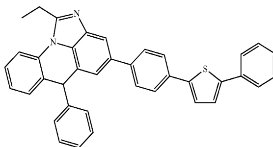
[Chemical Formula 10-4]
