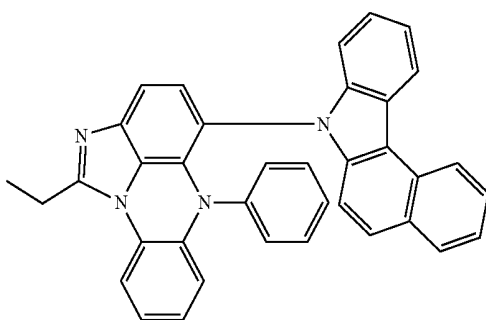
[Chemical Formula 9-15]
