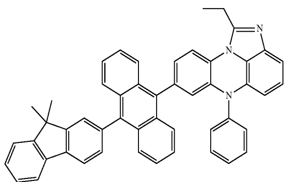
[Chemical Formula 3-6]
