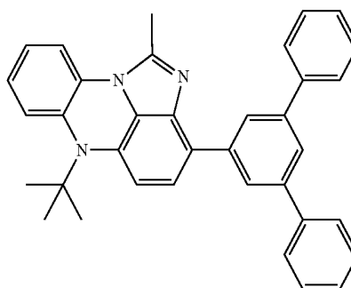
[Chemical Formula 11-4]
