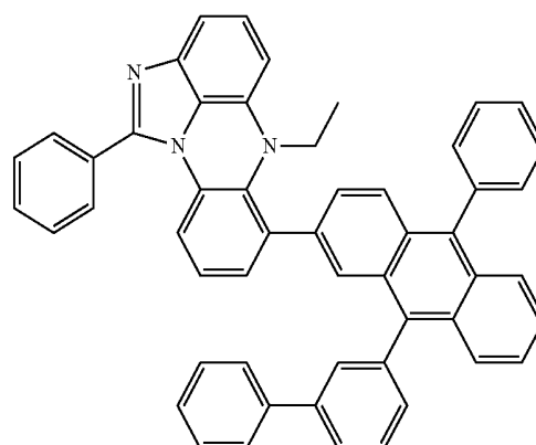
[Chemical Formula 6-24]
