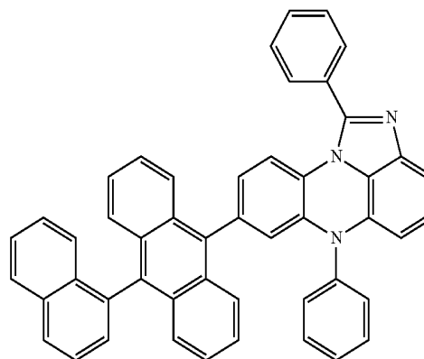
[Chemical Formula 4-3]
