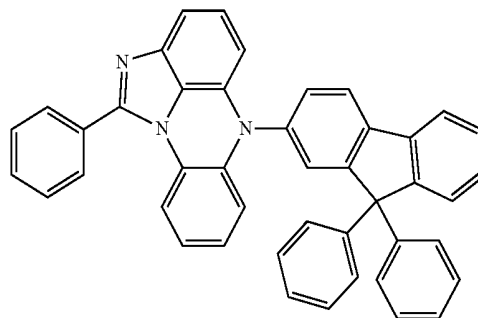
[Chemical Formula 12-35]
