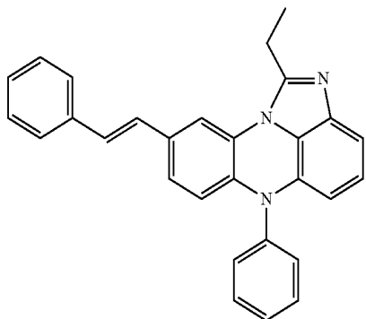
[Chemical Formula 7-54]
