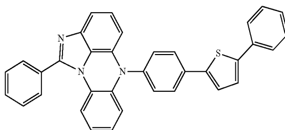
[Chemical Formula 12-39]
