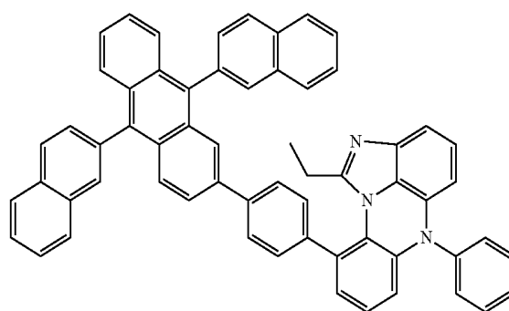
[Chemical Formula 8-25]
