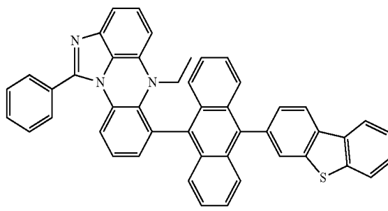
[Chemical Formula 6-14]
