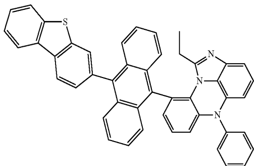
[Chemical Formula 8-14]
