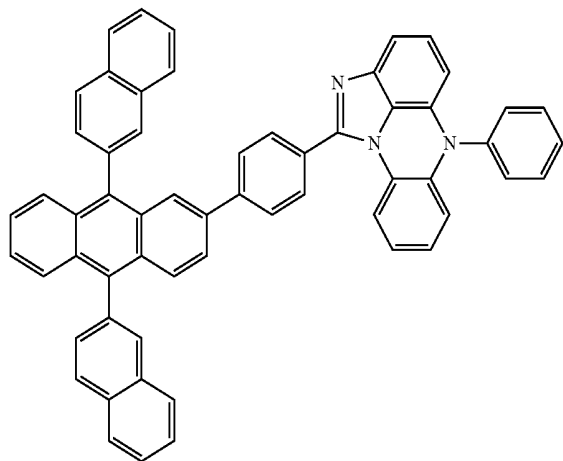
[Chemical Formula 5-25]
