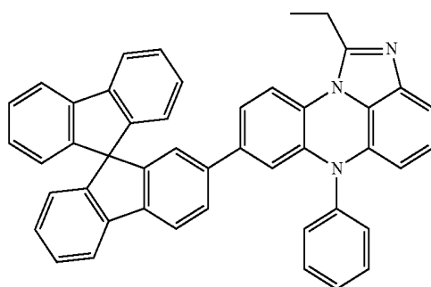
[Chemical Formula 3-34]
