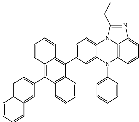
[Chemical Formula 3-3]
