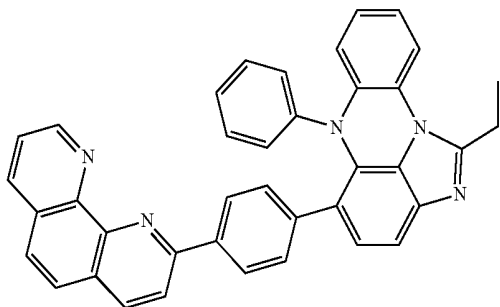
[Chemical Formula 9-12]
