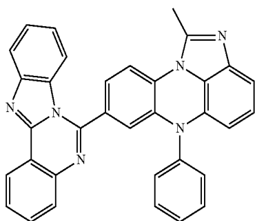
[Chemical Formula 2-53]
