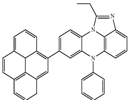
[Chemical Formula 3-28]
