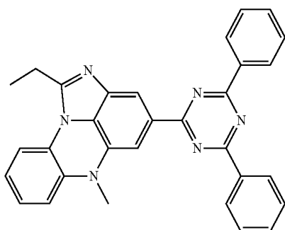
[Chemical Formula 10-6]
