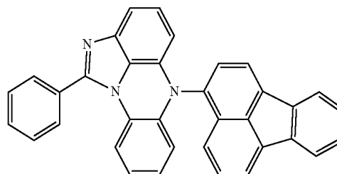
[Chemical Formula 12-30]
