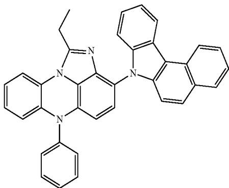
[Chemical Formula 11-15]
