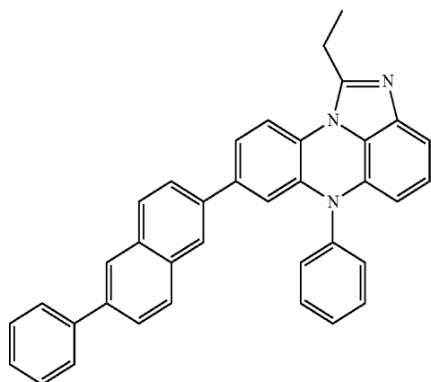
[Chemical Formula 3-27]
