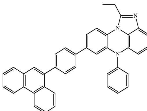
[Chemical Formula 3-31]
