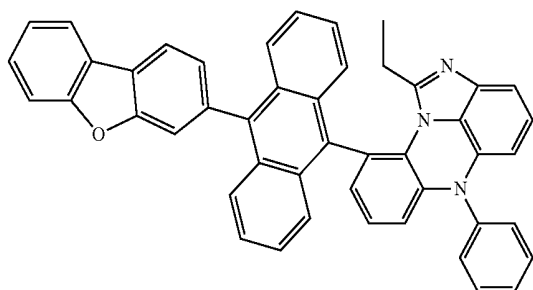
[Chemical Formula 8-13]
