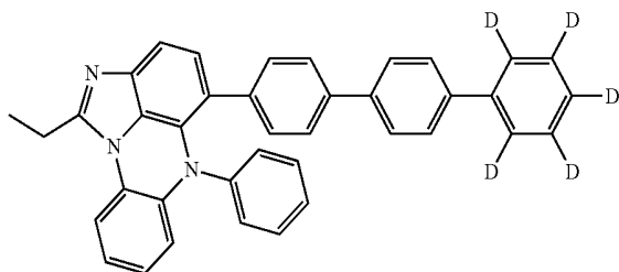
[Chemical Formula 9-16]
