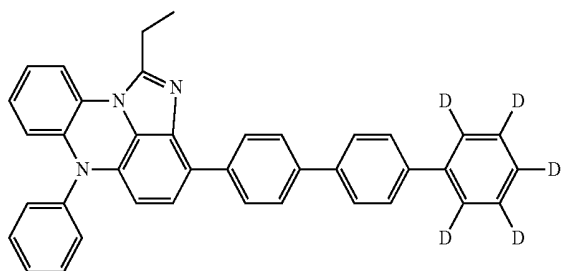
[Chemical Formula 11-16]
