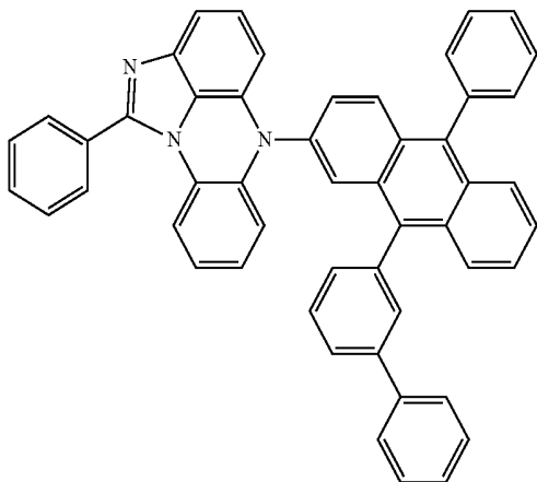
[Chemical Formula 12-24]
