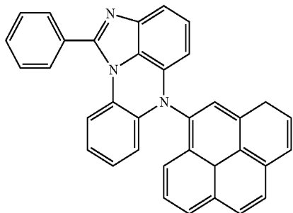
[Chemical Formula 12-29]
