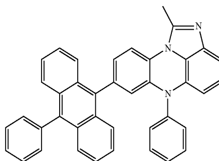
[Chemical Formula 2-2]
