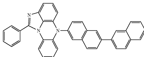
[Chemical Formula 12-45]
