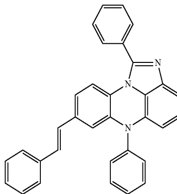
[Chemical Formula 4-54]
