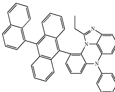
[Chemical Formula 8-3]
