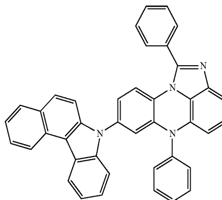
[Chemical Formula 4-52]
