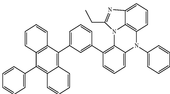
[Chemical Formula 8-18]
