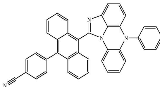
[Chemical Formula 5-12]
