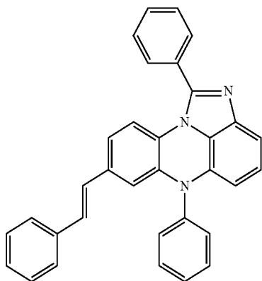
[Chemical Formula 4-54]
