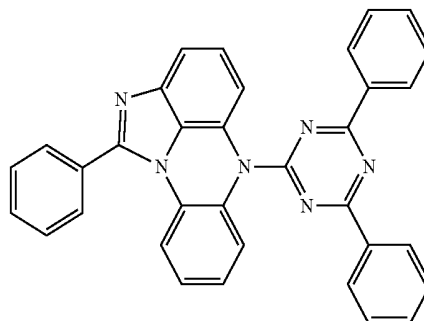
[Chemical Formula 12-42]
