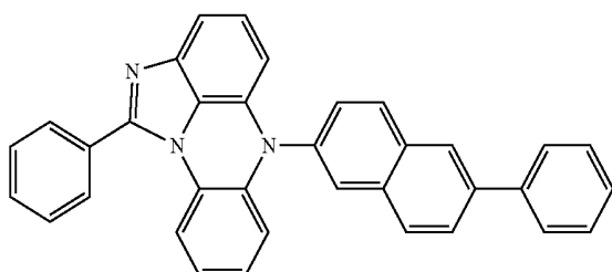
[Chemical Formula 12-27]
