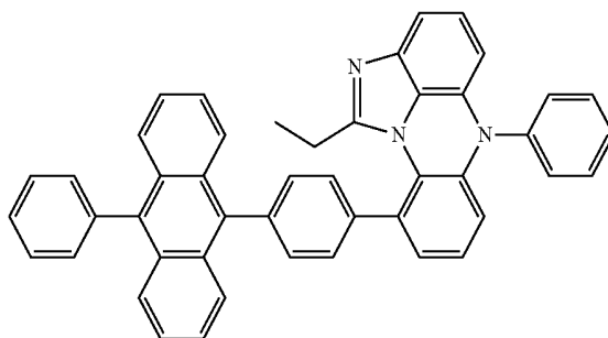
[Chemical Formula 8-17]
