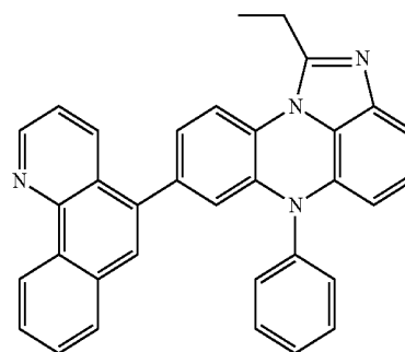
[Chemical Formula 3-33]
