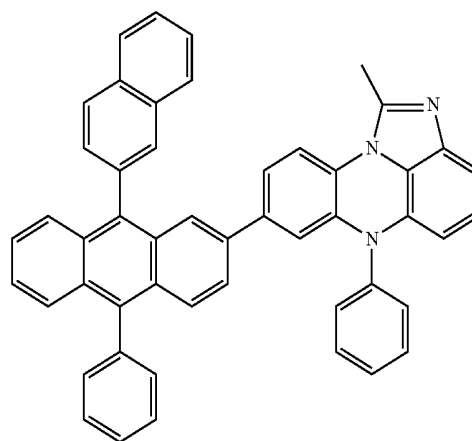
[Chemical Formula 2-23]
