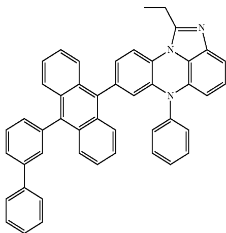
[Chemical Formula 3-7]
