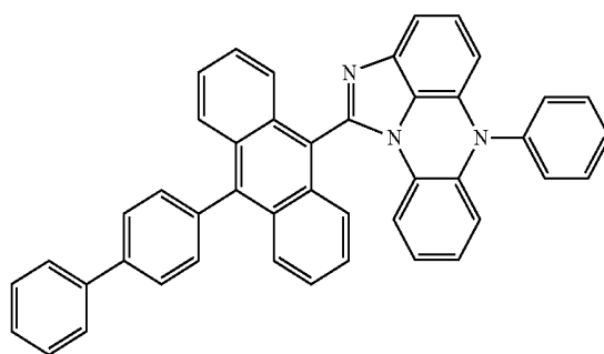
[Chemical Formula 5-4]
