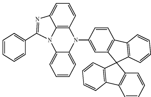
[Chemical Formula 12-34]
