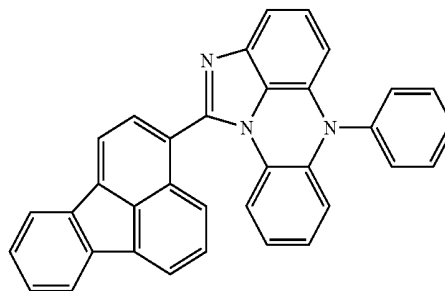
[Chemical Formula 5-30]
