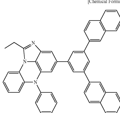
[Chemical Formula 10-8]
