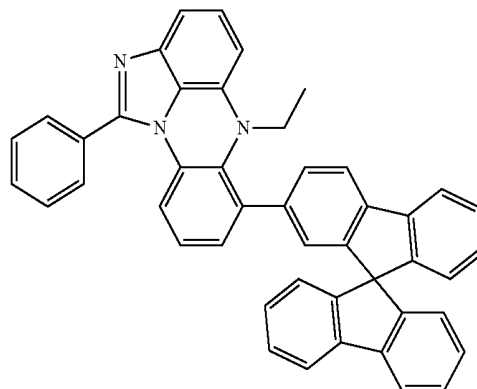
[Chemical Formula 6-34]
