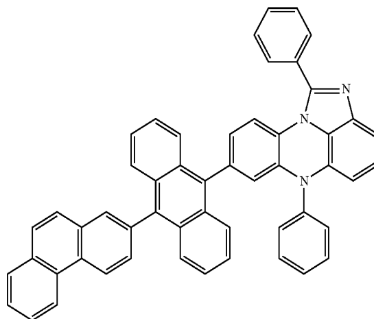
[Chemical Formula 4-9]
