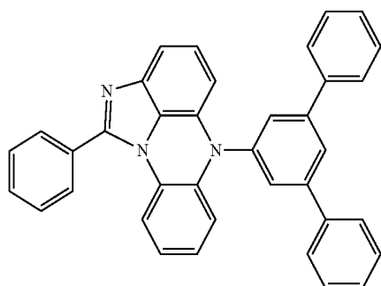
[Chemical Formula 12-40]
