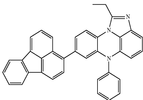
[Chemical Formula 3-30]
