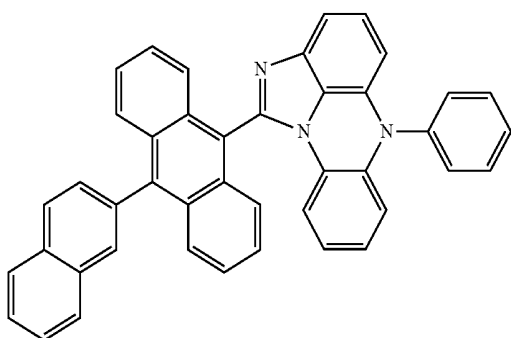
[Chemical Formula 5-2]
