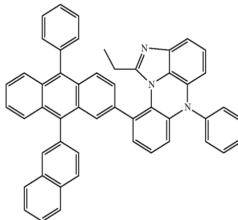
[Chemical Formula 8-23]
