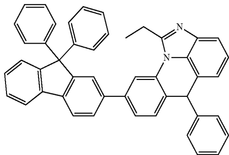
[Chemical Formula 7-35]
