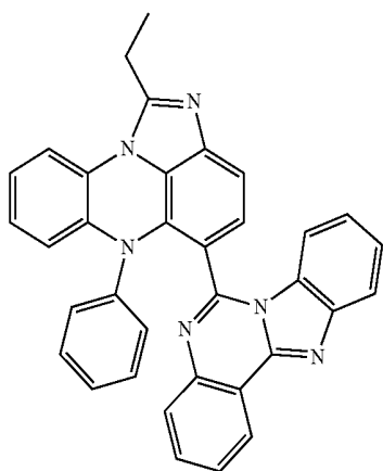
[Chemical Formula 9-17]
