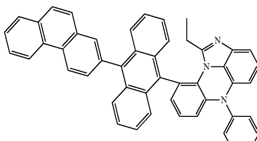
[Chemical Formula 8-10]
