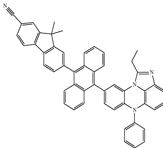
[Chemical Formula 7-15]
