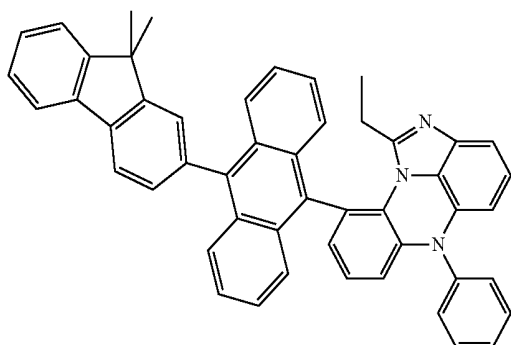
[Chemical Formula 8-5]
