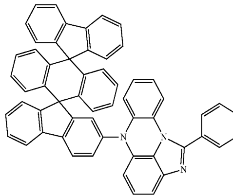
[Chemical Formula 12-36]
