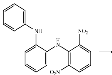
[Compound 18-A]
