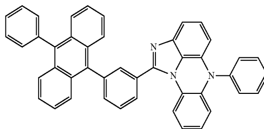
[Chemical Formula 5-18]
