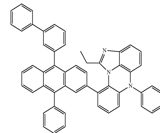
[Chemical Formula 8-25]
