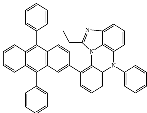
[Chemical Formula 8-19]
