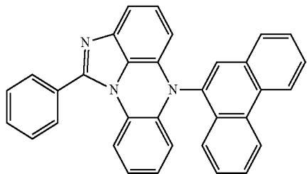
[Chemical Formula 12-31]
