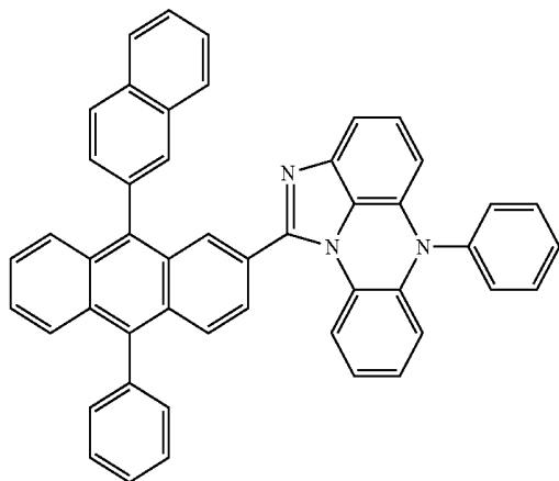
[Chemical Formula 5-23]
