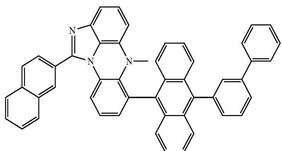
[Chemical Formula 6-7]
