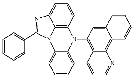
[Chemical Formula 12-33]
