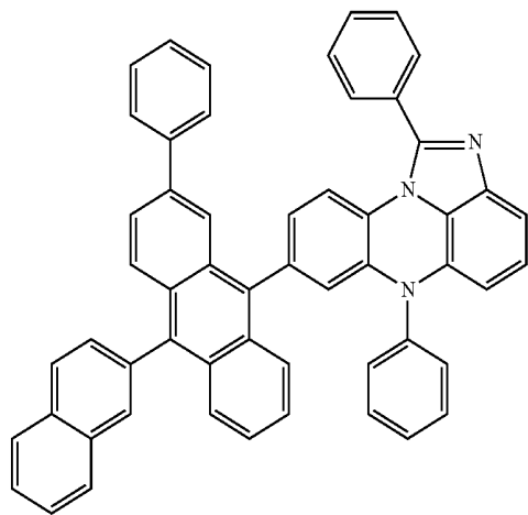
[Chemical Formula 4-16]
