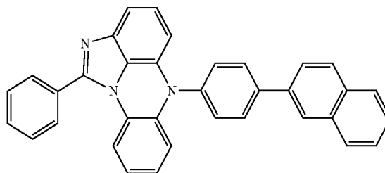
[Chemical Formula 12-26]
