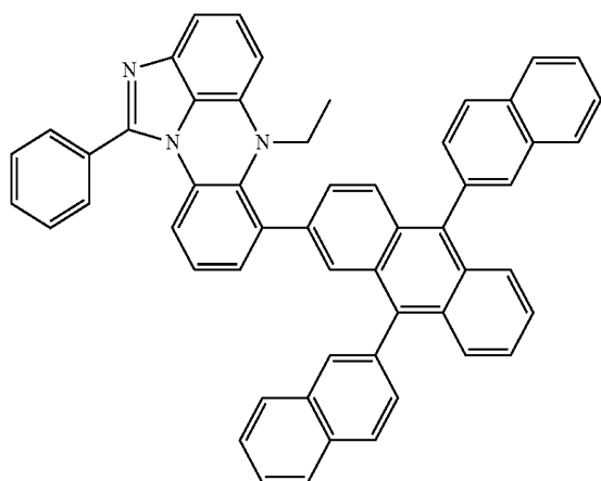
[Chemical Formula 6-20]
