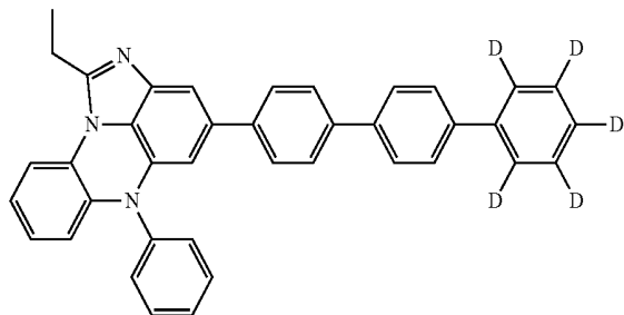
[Chemical Formula 10-16]
