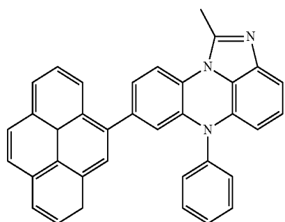
[Chemical Formula 2-28]
