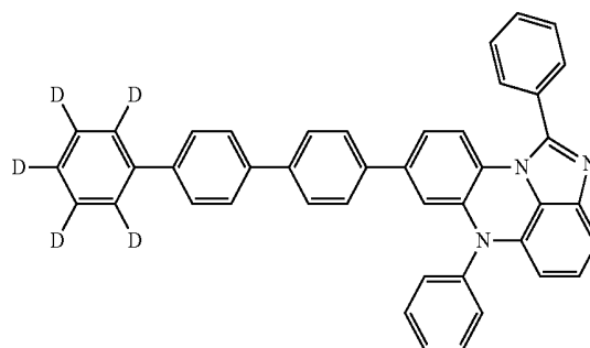
[Chemical Formula 4-52]
