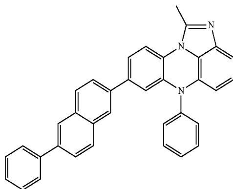
[Chemical Formula 2-28]
