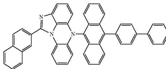
[Chemical Formula 12-4]
