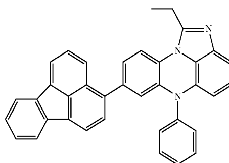
[Chemical Formula 3-30]
