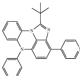
[Chemical Formula 11-2]
