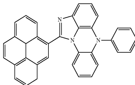
[Chemical Formula 5-29]
