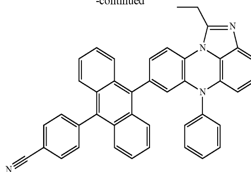
[Chemical Formula 3-12]
