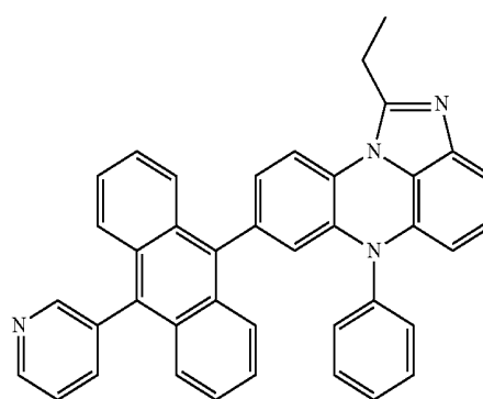
[Chemical Formula 3-11]
