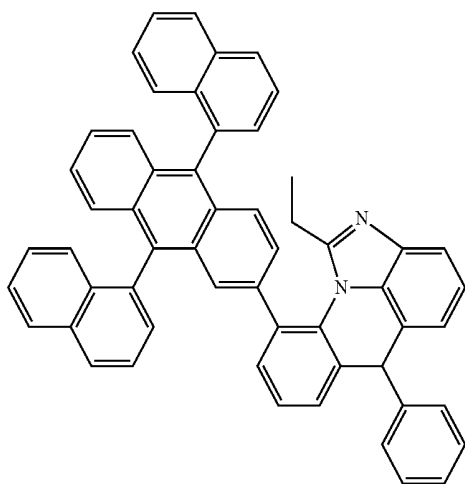
[Chemical Formula 8-21]
