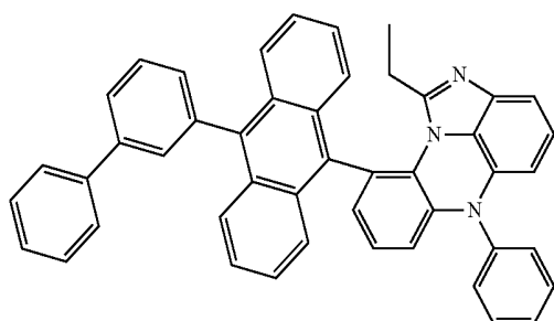
[Chemical Formula 8-6]
