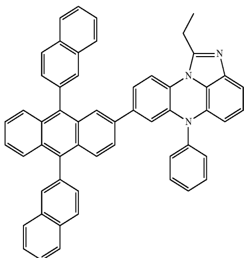
[Chemical Formula 3-20]
