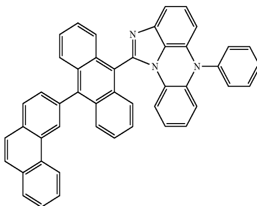
[Chemical Formula 5-8]
