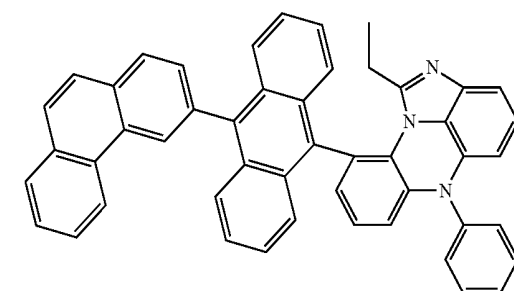
[Chemical Formula 8-9]
