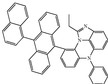
[Chemical Formula 8-3]
