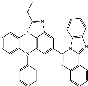
[Chemical Formula 10-17]
