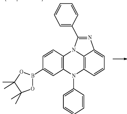
[Compound 17-A]
