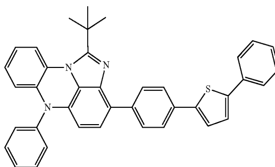
[Chemical Formula 11-3]
