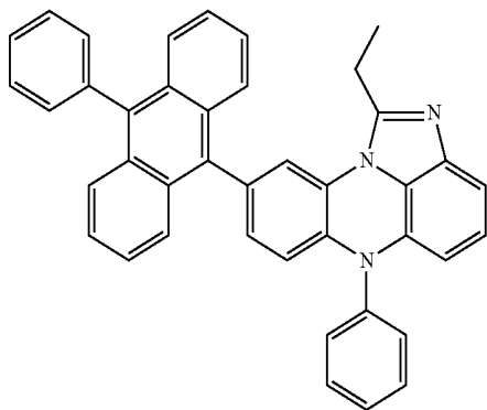
[Chemical Formula 7-1]
