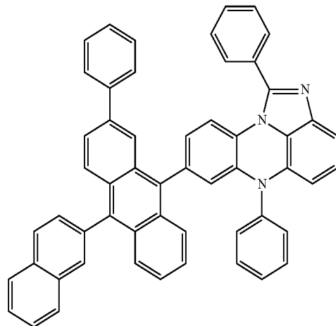
[Chemical Formula 4-16]
