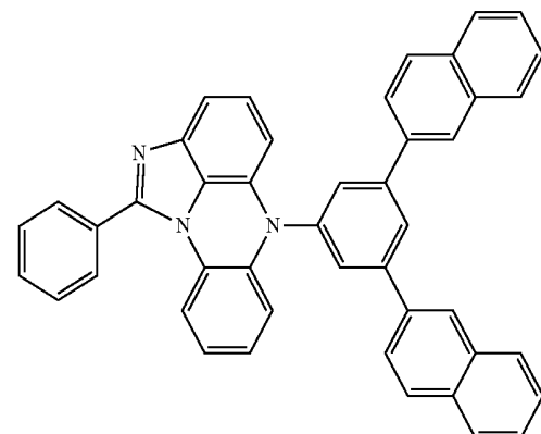
[Chemical Formula 12-44]
