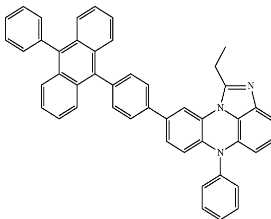
[Chemical Formula 7-17]
