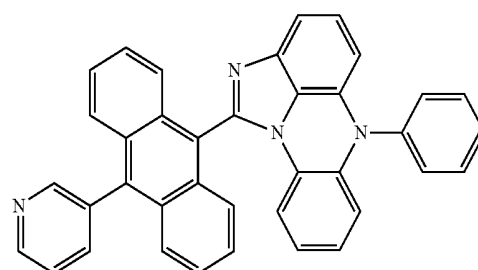
[Chemical Formula 5-10]
