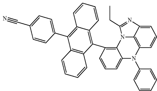
[Chemical Formula 8-12]
