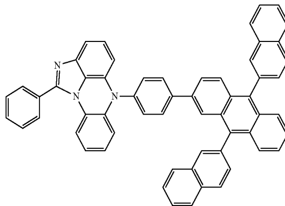
[Chemical Formula 12-25]
