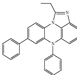
[Chemical Formula 3-33]
