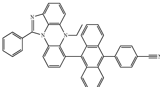
[Chemical Formula 6-13]
