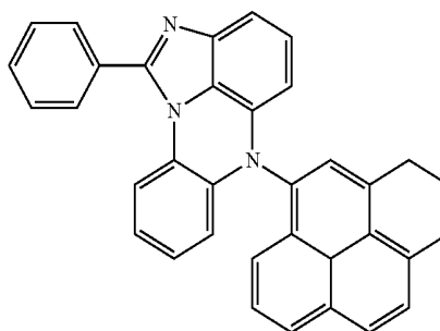
[Chemical Formula 12-29]
