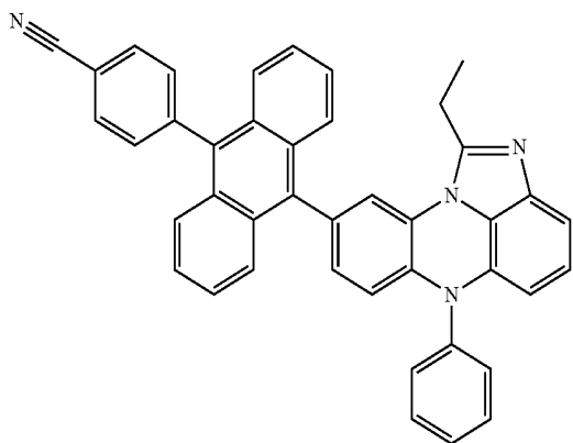
[Chemical Formula 7-12]
