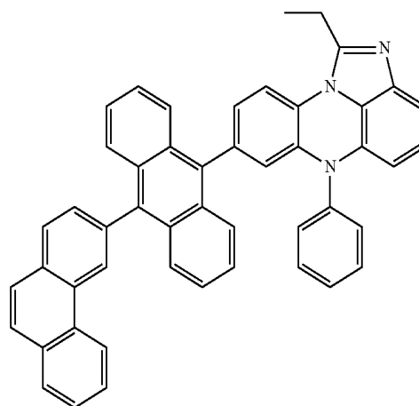
[Chemical Formula 3-8]
