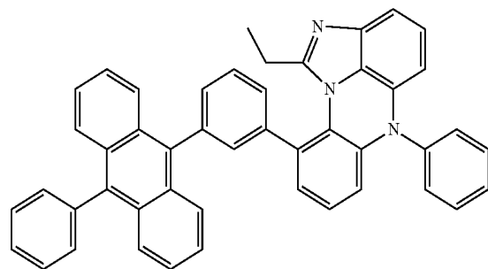
[Chemical Formula 8-18]
