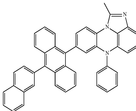
[Chemical Formula 2-2]
