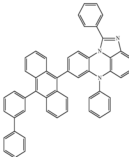
[Chemical Formula 4-6]
