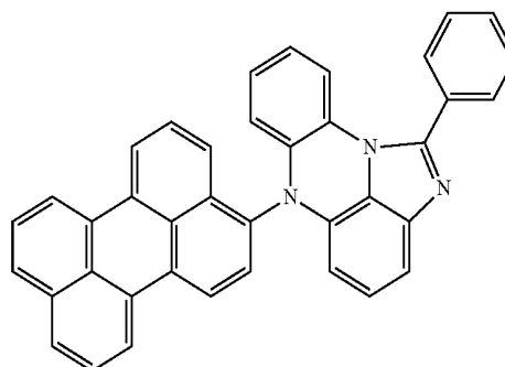
[Chemical Formula 12-29]
