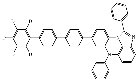
[Chemical Formula 4-53]
