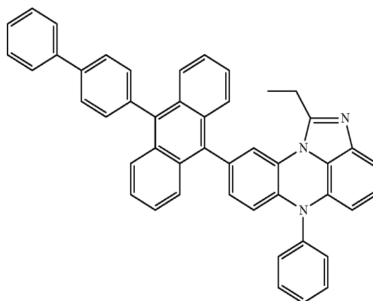
[Chemical Formula 7-4]
