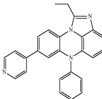
[Chemical Formula 3-34]
