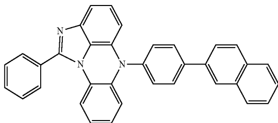
[Chemical Formula 12-26]
