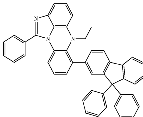
[Chemical Formula 6-35]
