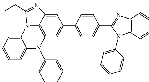
[Chemical Formula 10-10]
