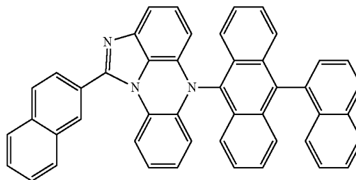
[Chemical Formula 12-3]
