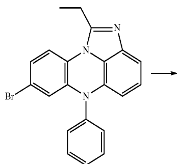
[Compound 2-A]
