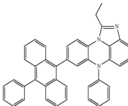
[Chemical Formula 3-1]
