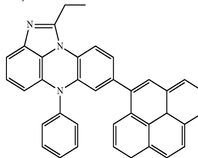
[Chemical Formula 3-28]
