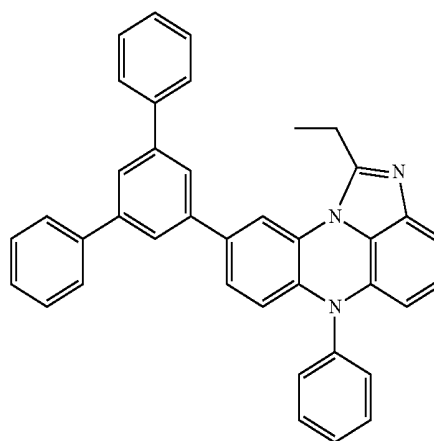
[Chemical Formula 7-40]
