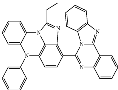
[Chemical Formula 11-17]
