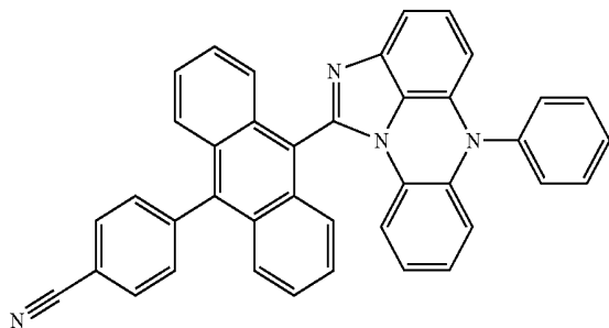
[Chemical Formula 5-12]
