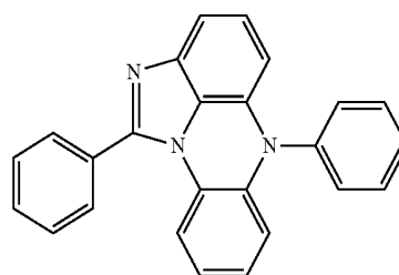
[Chemical Formula 5-37]
