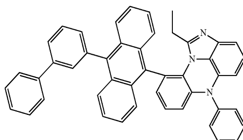
[Chemical Formula 8-6]
