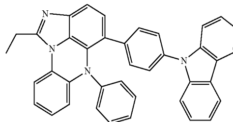
[Chemical Formula 9-6]
