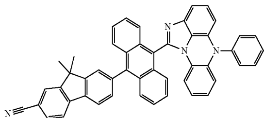
[Chemical Formula 5-15]
