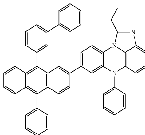
[Chemical Formula 3-24]
