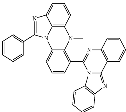
[Chemical Formula 6-53]
