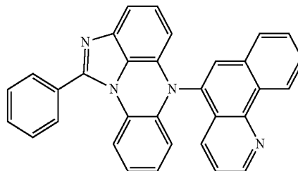
[Chemical Formula 12-33]
