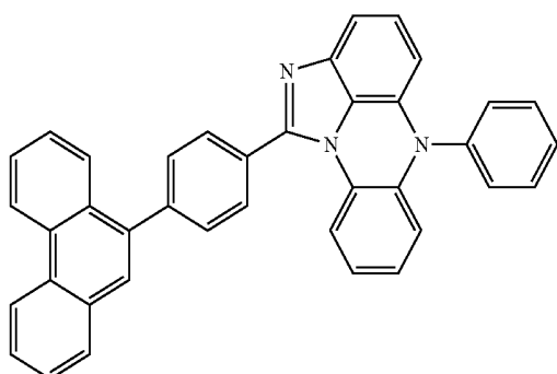
[Chemical Formula 5-32]
