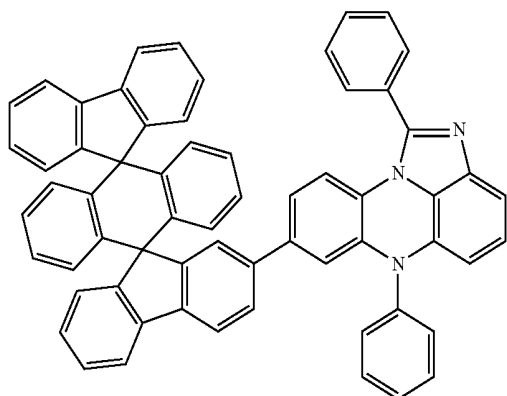
[Chemical Formula 4-37]
