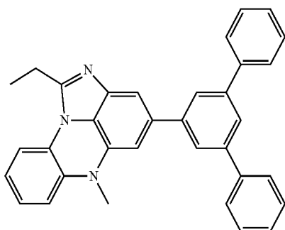
[Chemical Formula 10-5]
