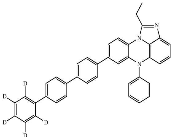
[Chemical Formula 3-53]
