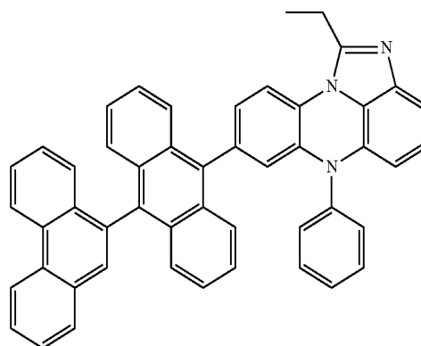
[Chemical Formula 3-7]
