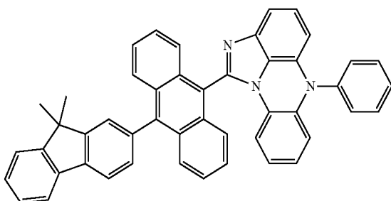
[Chemical Formula 5-5]
