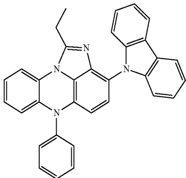
[Chemical Formula 11-14]
