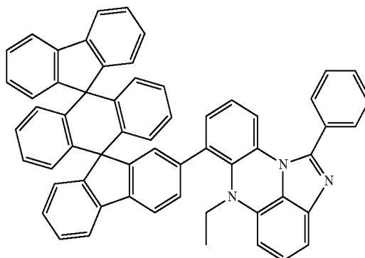
[Chemical Formula 6-36]
