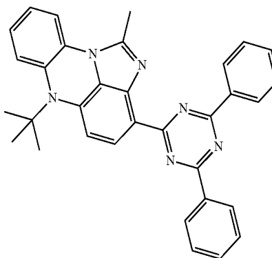
[Chemical Formula 11-5]
