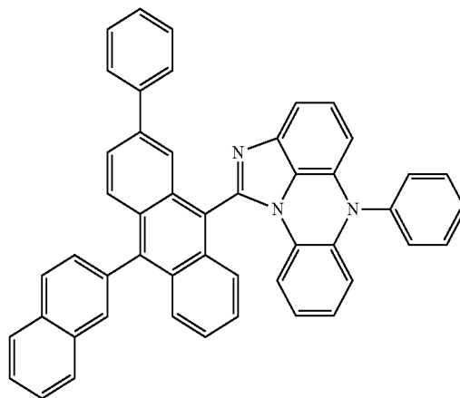
[Chemical Formula 5-16]
