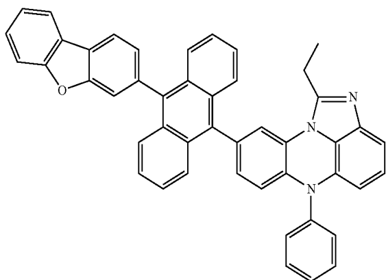
[Chemical Formula 7-13]
