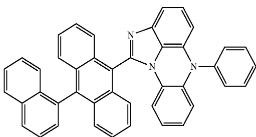
[Chemical Formula 5-3]
