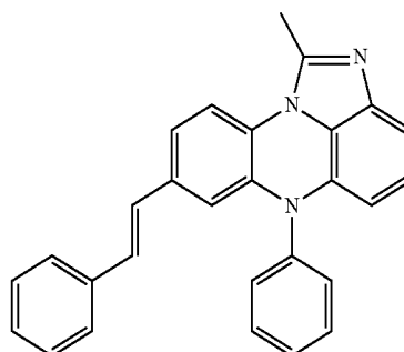
[Chemical Formula 2-54]
