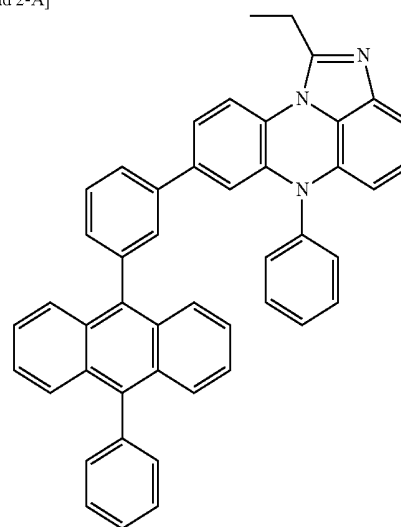
[Chemical Formula 3-18]
