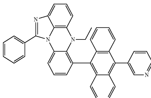
[Chemical Formula 6-11]
