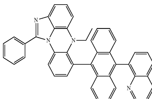
[Chemical Formula 6-12]
