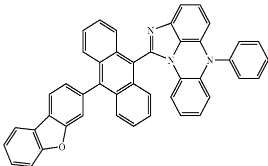
[Chemical Formula 5-13]
