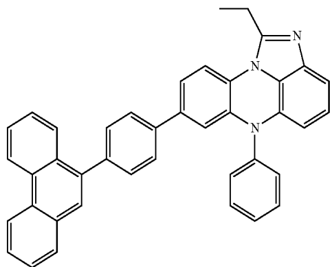
[Chemical Formula 3-32]
