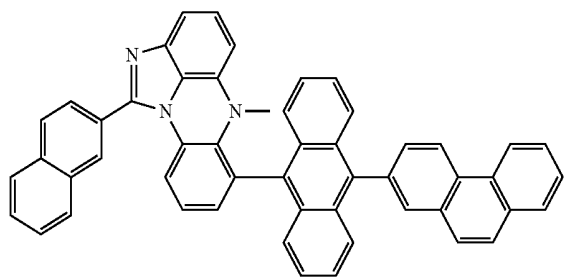
[Chemical Formula 6-9]
