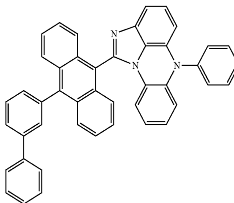
[Chemical Formula 5-6]
