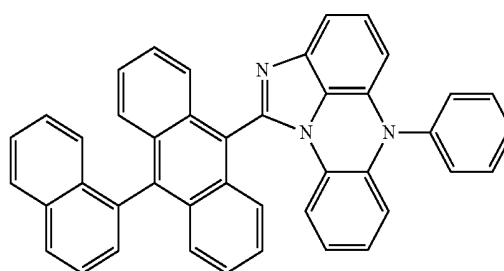
[Chemical Formula 5-3]
