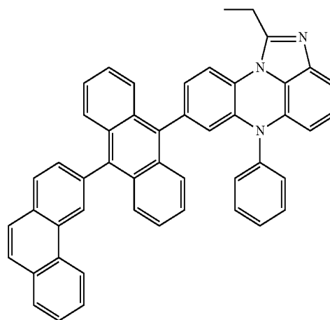
[Chemical Formula 3-9]
