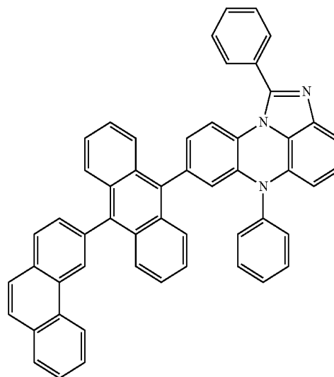
[Chemical Formula 4-8]
