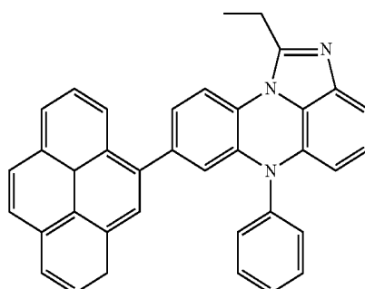
[Chemical Formula 3-28]
