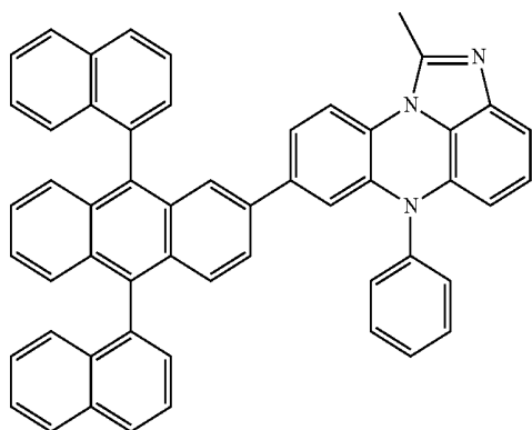
[Chemical Formula 2-21]
