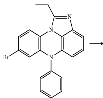
[Compound 2-A]
