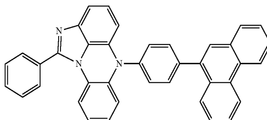
[Chemical Formula 12-32]
