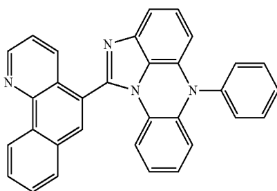
[Chemical Formula 5-33]
