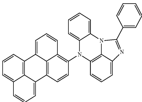
[Chemical Formula 12-29]
