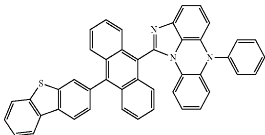
[Chemical Formula 5-14]
