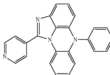
[Chemical Formula 5-38]
