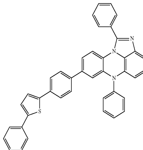
[Chemical Formula 4-39]
