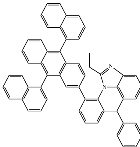
[Chemical Formula 8-21]
