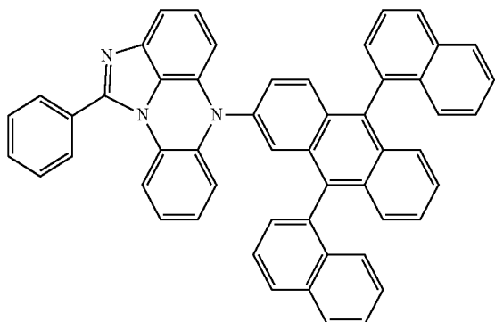
[Chemical Formula 12-22]
