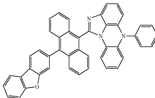
[Chemical Formula 5-13]
