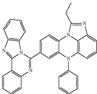
[Chemical Formula 3-53]
