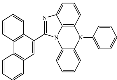
[Chemical Formula 5-31]
