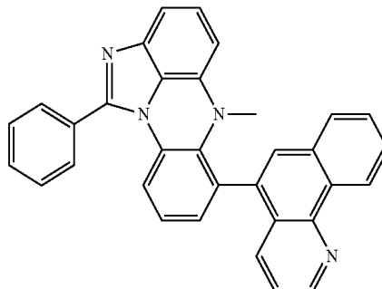
[Chemical Formula 6-34]
