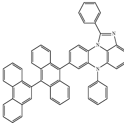
[Chemical Formula 4-7]
