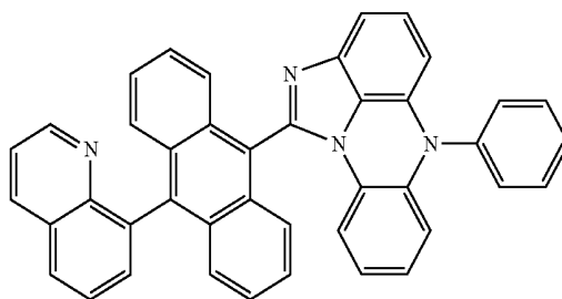
[Chemical Formula 5-11]
