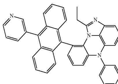
[Chemical Formula 8-11]
