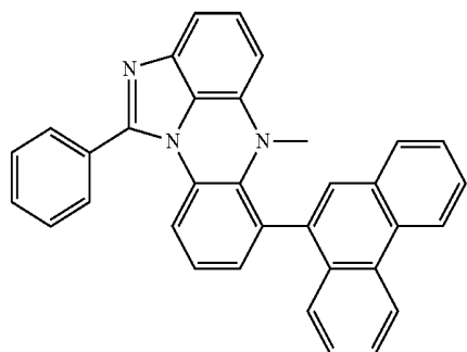
[Chemical Formula 6-31]
