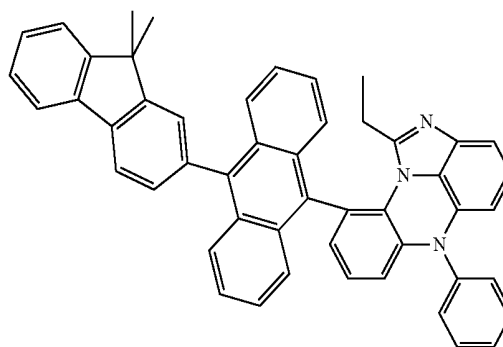
[Chemical Formula 8-5]
