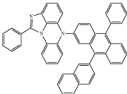
[Chemical Formula 12-23]
