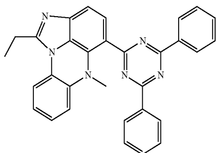
[Chemical Formula 9-5]
